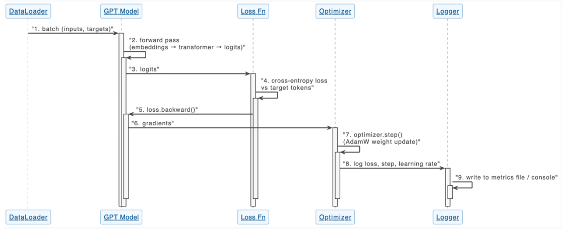
Figure 5: Sequence Diagram - One Training Iteration
