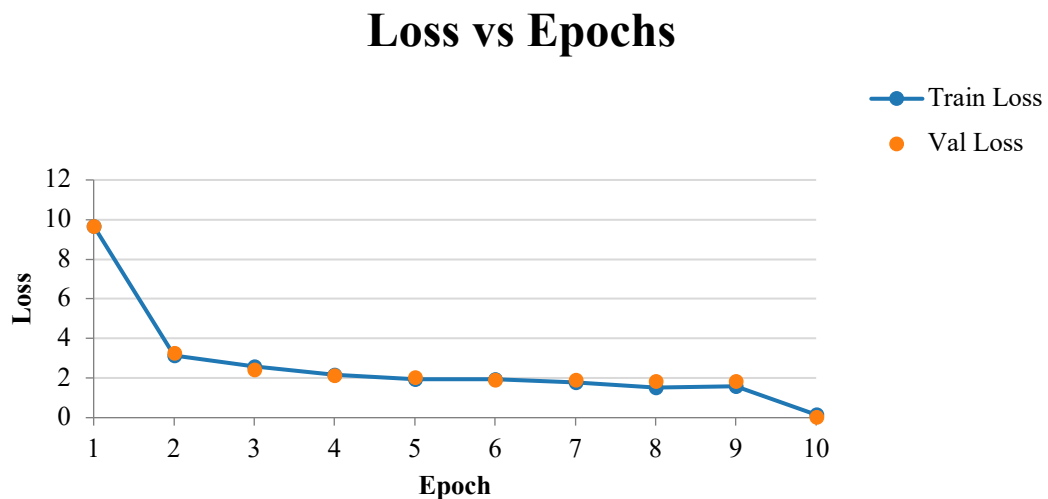
Figure 10: Loss vs Epochs (Illustrative Training Curve)
